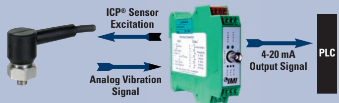
ICP® Accelerometer
